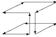
Fig. 1. Covariant derivatives around a cube.
