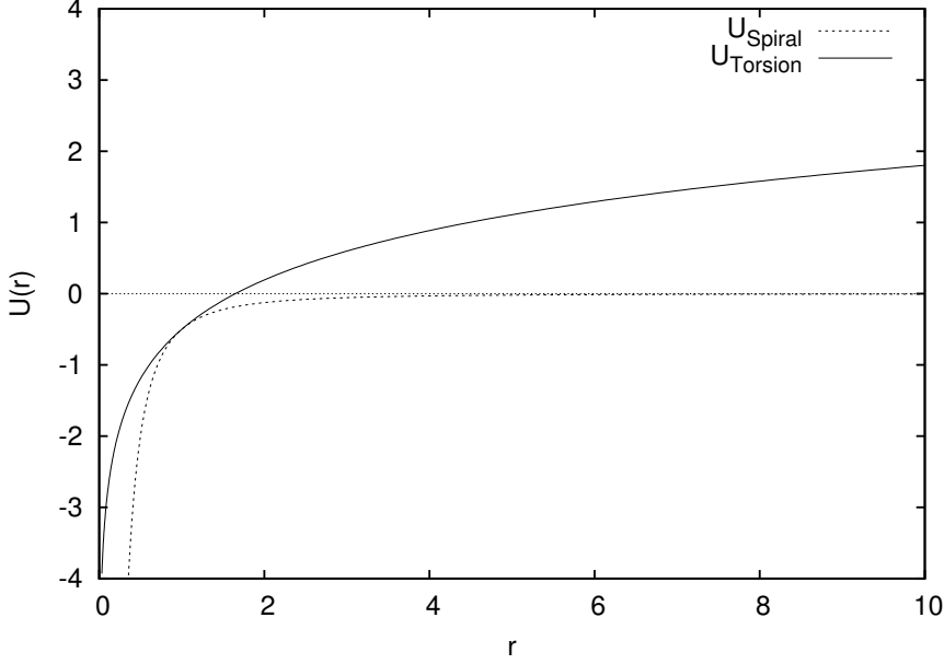
Figure 1.7: Potential for radius-dependent \alpha , model of Eq. (1.58).
