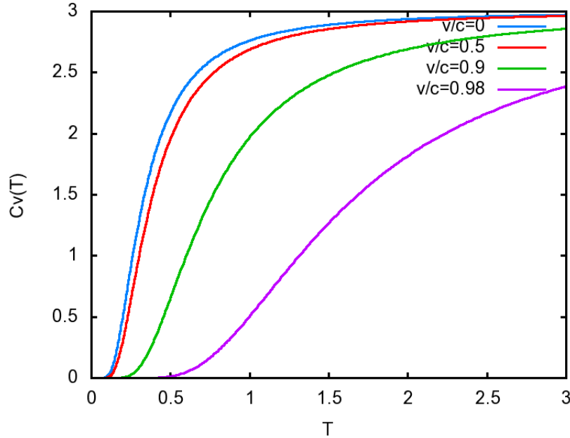
Figure 1: Function C_v(T) for different ratios v/c .
